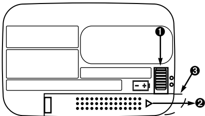
Advisor Pro Rear View (Battery Replacement)
